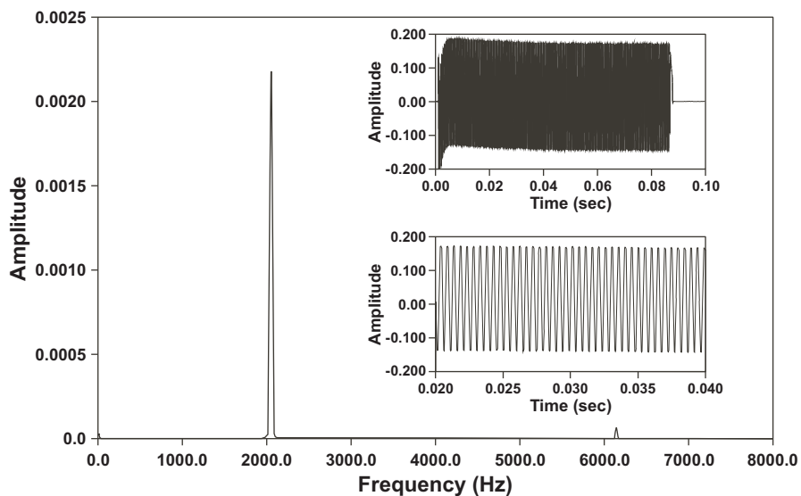
Fig. 3. Frequency spectrum and the microphone recorded squeal signal when a 56 mm long chalk was rubbed on a small irregularly shaped ceramic plate, roughly 30 \times 25 mm by 5 mm thick. f_d \approx 2050 Hz.
