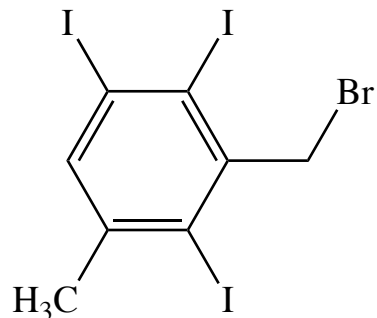
3-bromomethyl- 1,2,4-triiodo 5-methylbenzene
