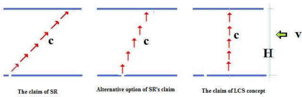
Fig. 3 The path of photon on a moving body
