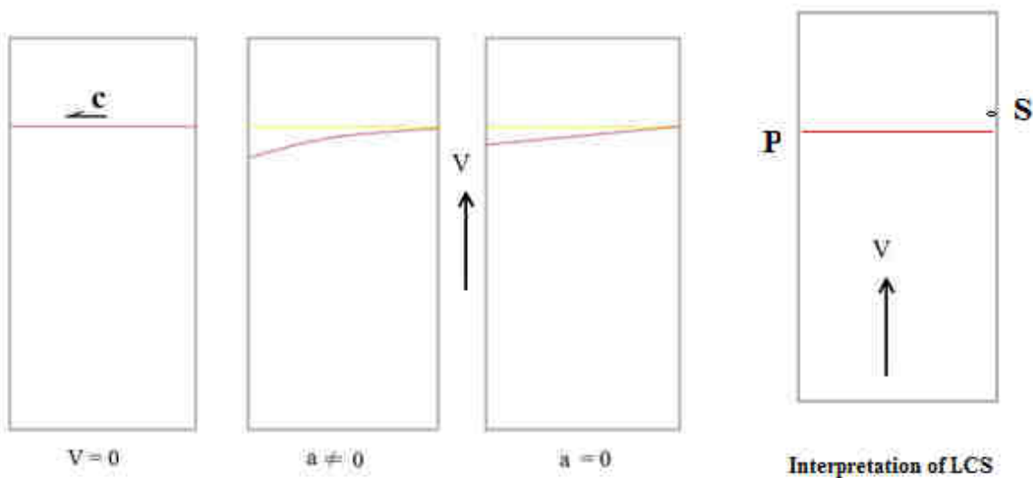
Fig. 4. The path of horizontal light in an elevator cabinet
