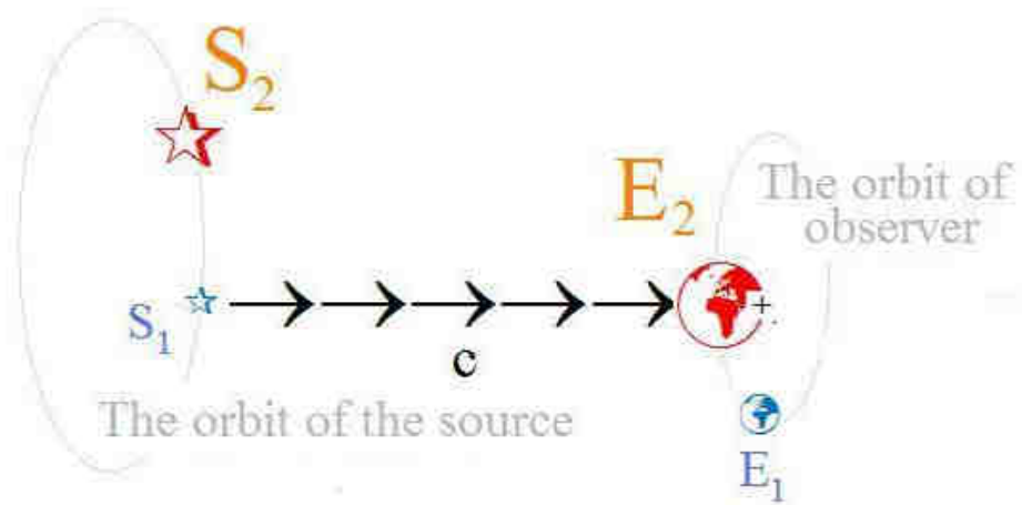
Figure The emitting point of a photon is marked on outer space or LCS
