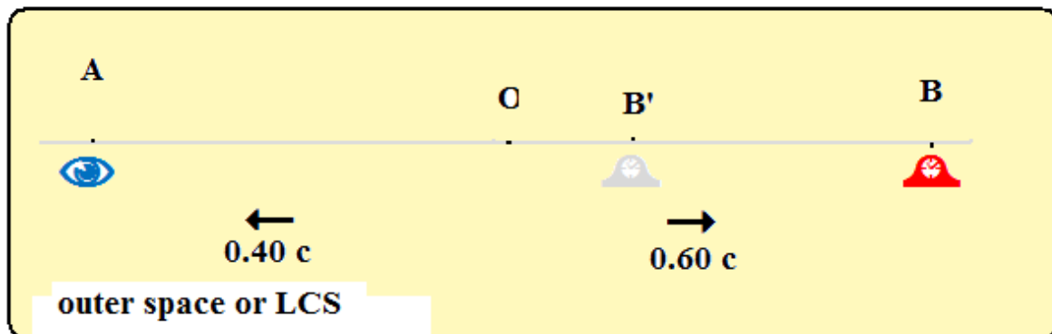
Figure: An observer can see deformed position and time
