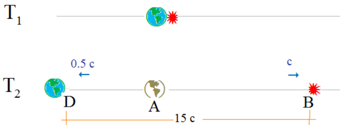
Figure 2- The velocity of light is always measured as the value c
