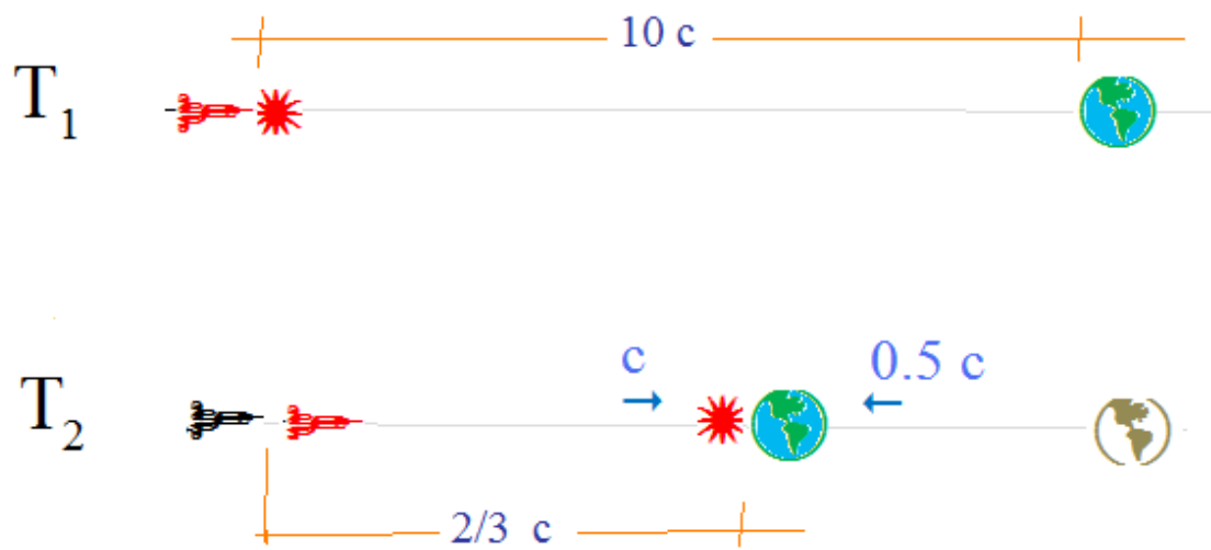
Figure 1- The light always arrives to an observer with the velocity of light c
