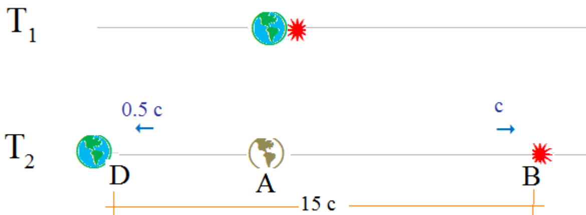
Figure 2- The velocity of light is always measured as the value c T = 10 inert second
